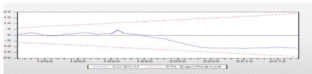
Fig.4: Recursive Test
